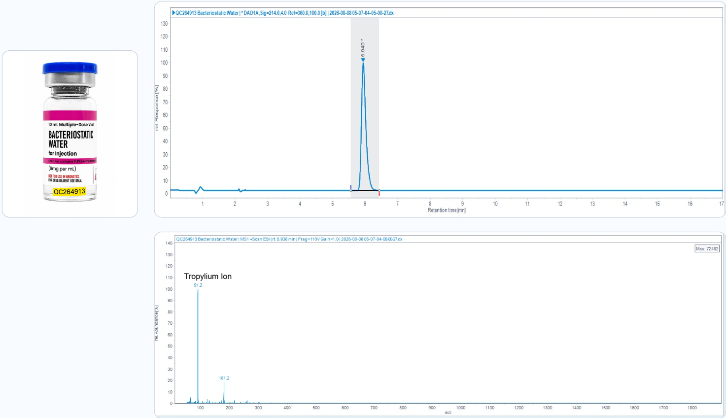
HPLC Chromatogram (Retention Time: 5.940 min)
